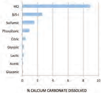
CALCIUM CARBONATE DISSOLVING PROPERTIES OF ACIDS: 3 MINUTE EXPOSURE (SURFACE SCALE REMOVAL)
