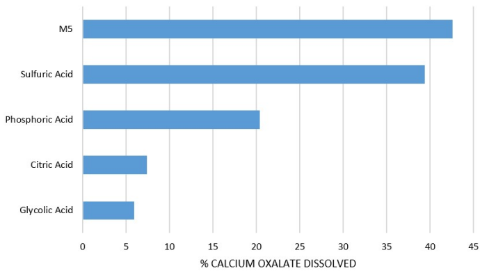
CALCIUM OXALATE DISSOLVING PROPERTIES OF ACIDS 5 MINUTE EXPOSURE (Recirculating Scale Removal)
