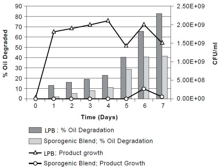
Motor Oil Degradation in a Parts Washer using LPB (10,000 ppm oil initially)
