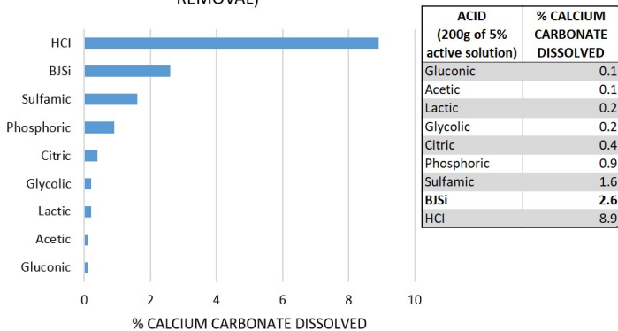
CALCIUM CARBONATE DISSOLVING PROPERTIES OF ACIDS: 3 MINUTE EXPOSURE (SURFACE SCALE REMOVAL)
